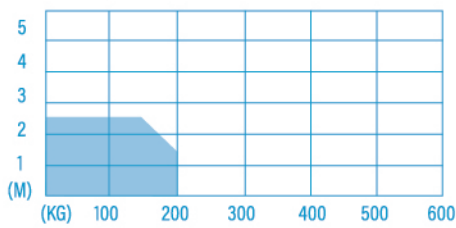
PW 220/220K
